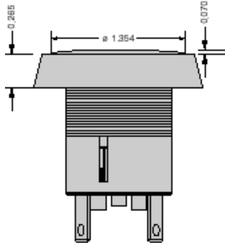
Standard Version Maintained and Momentary
