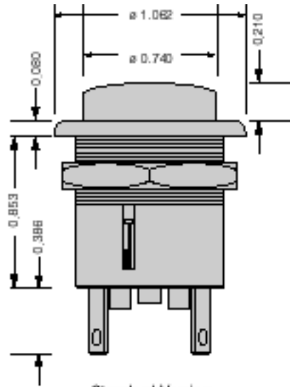
Standard Version Maintained and Momentary
